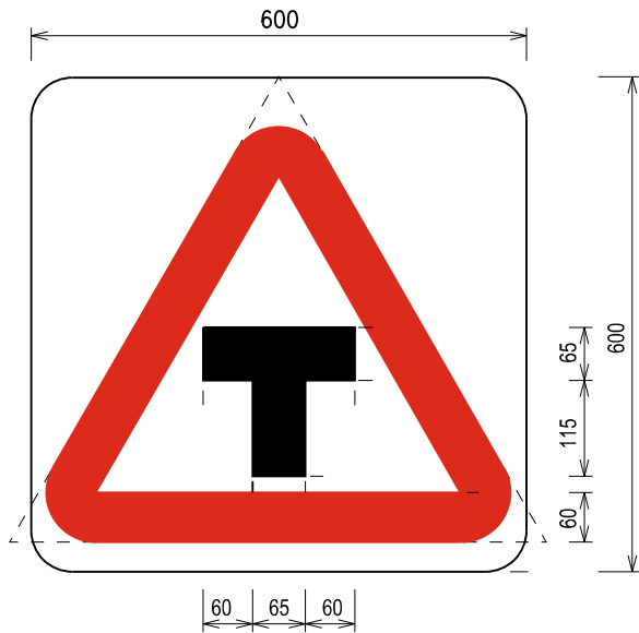
T-JUNCTION AHEAD
