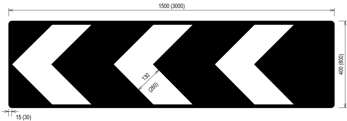
SHARP DEVIATION
