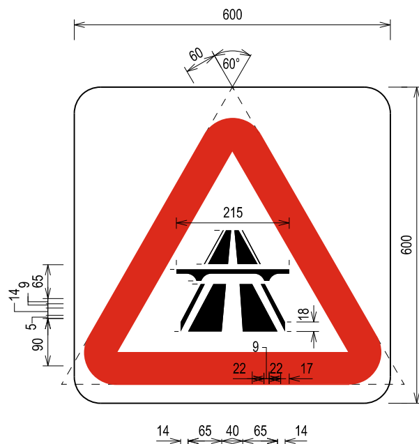
EXPRESSWAY AHEAD
