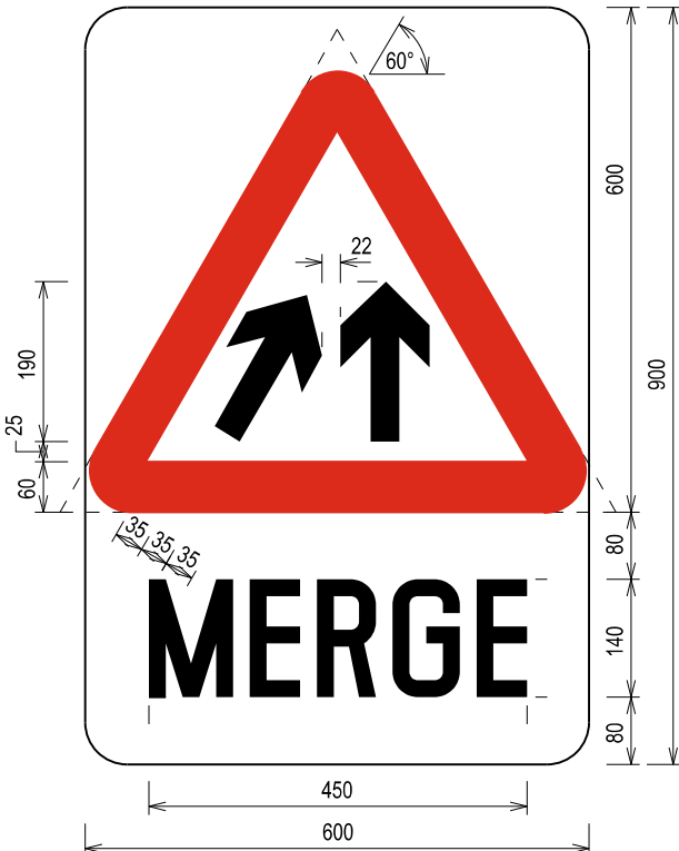
MERGE AHEAD
