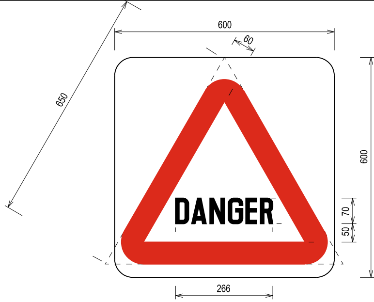
DANGER AHEAD
