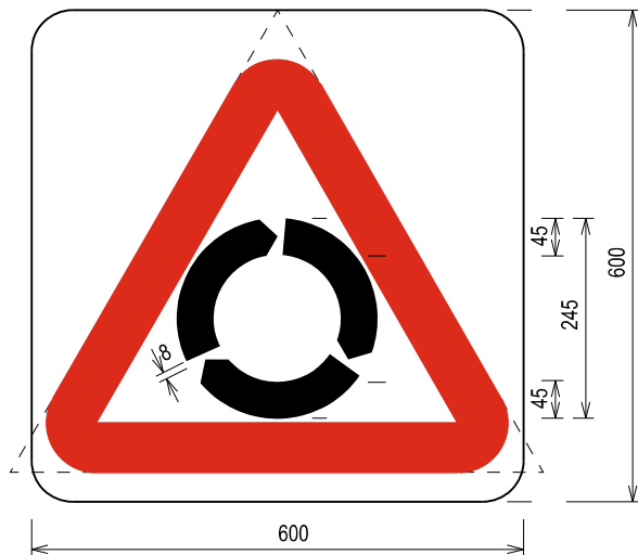
ROUNDABOUT AHEAD
