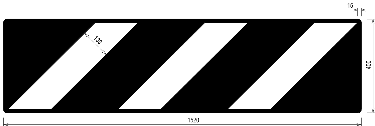
BARRIER
